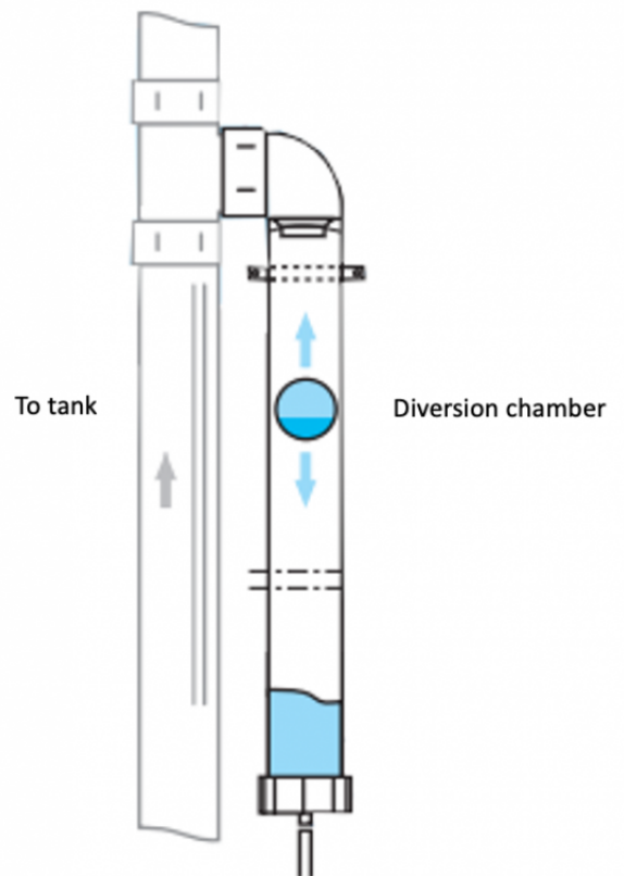
Wet System (right at tank)
