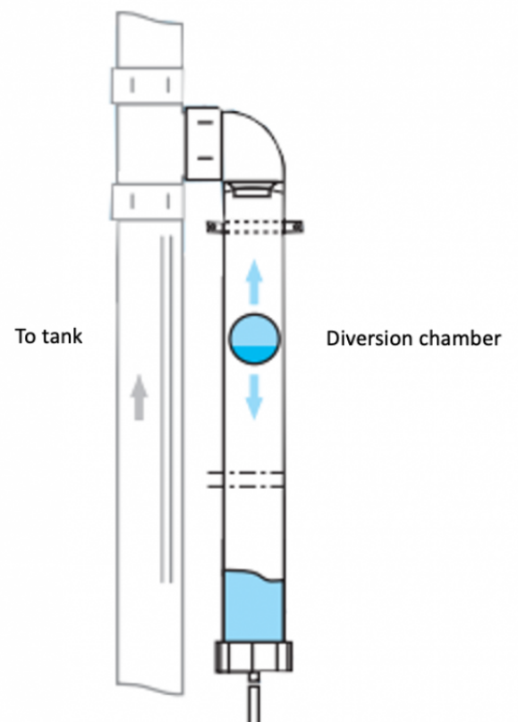
Wet System (right at tank)
