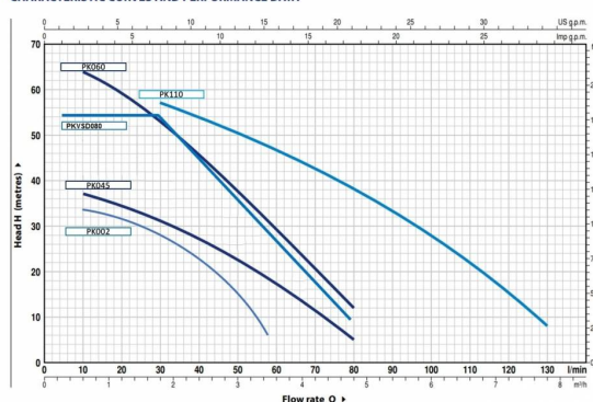
CHARACTERISTIC CURVES AND PERFORMANCE DATA
